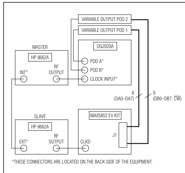
Figure 1. MAX5852 EV Kit Quick-Start Setup
